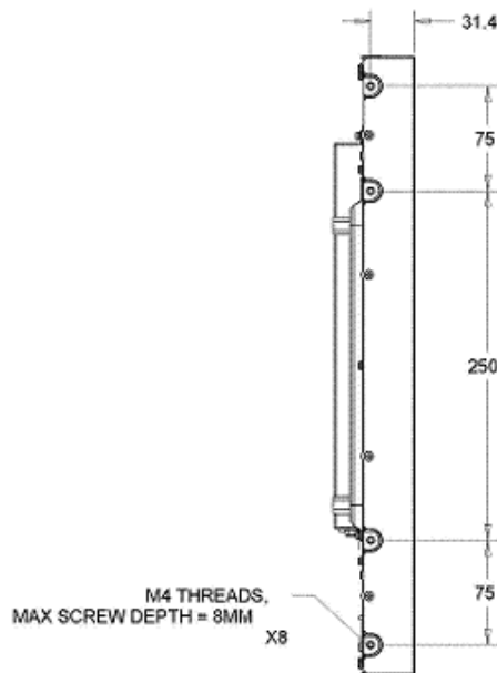
SIDE MOUNT VERTICAL (LEFT/RIGHT)
